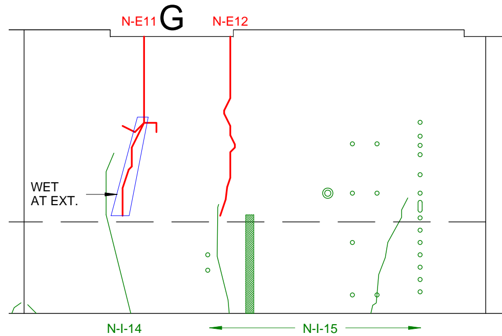
4 INT. PANEL 5 1/8" = 1'-0"
