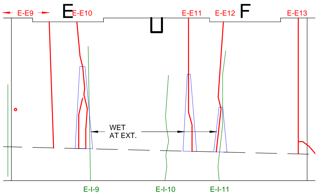
3 INT. PANEL 31 1/8" = 1'-0"
