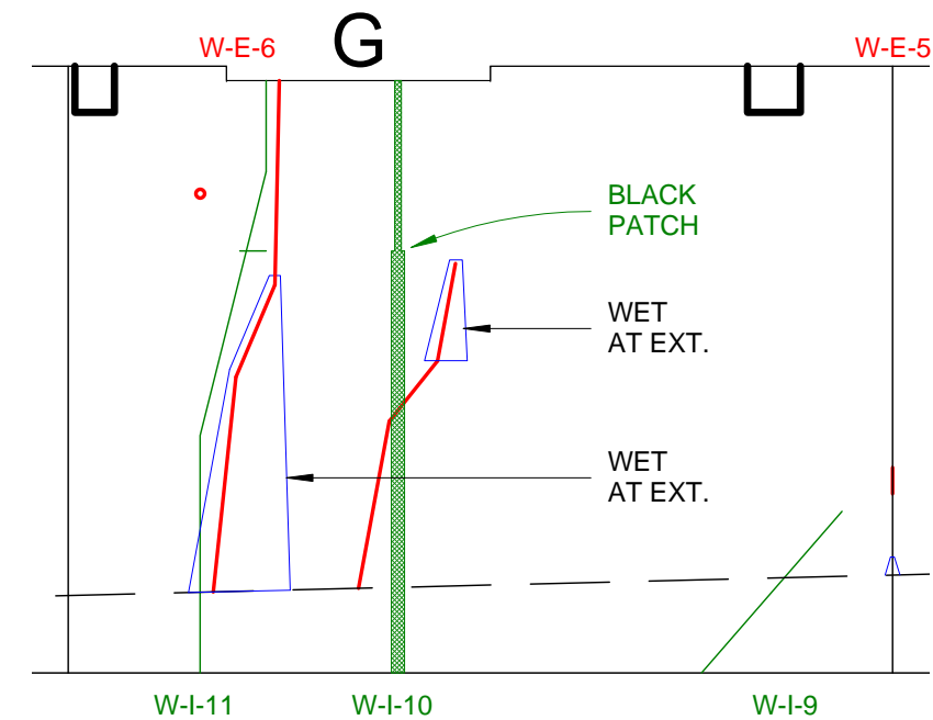
7 INT. PANEL 18 1/8" = 1'-0"
