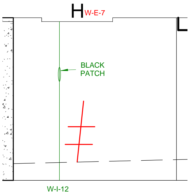
8 INT. PANEL 19 1/8" = 1'-0"
