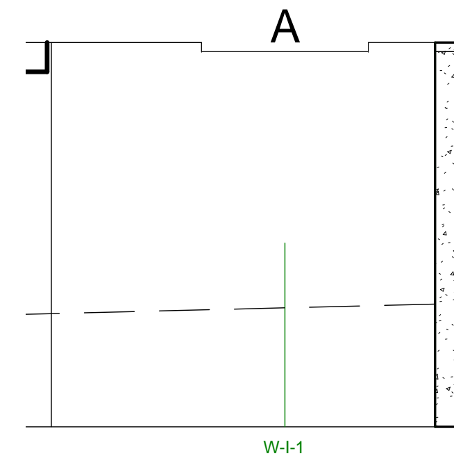
2 INT. PANEL 13 1/8" = 1'-0"
