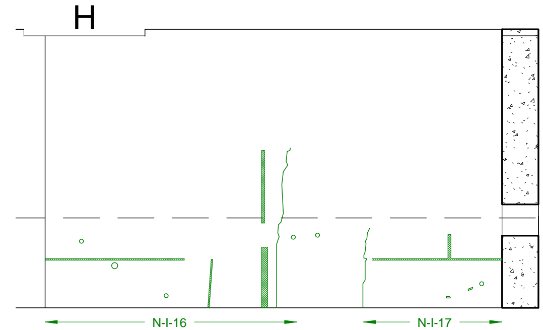
3 INT. PANEL 4 1/8" = 1'-0"
