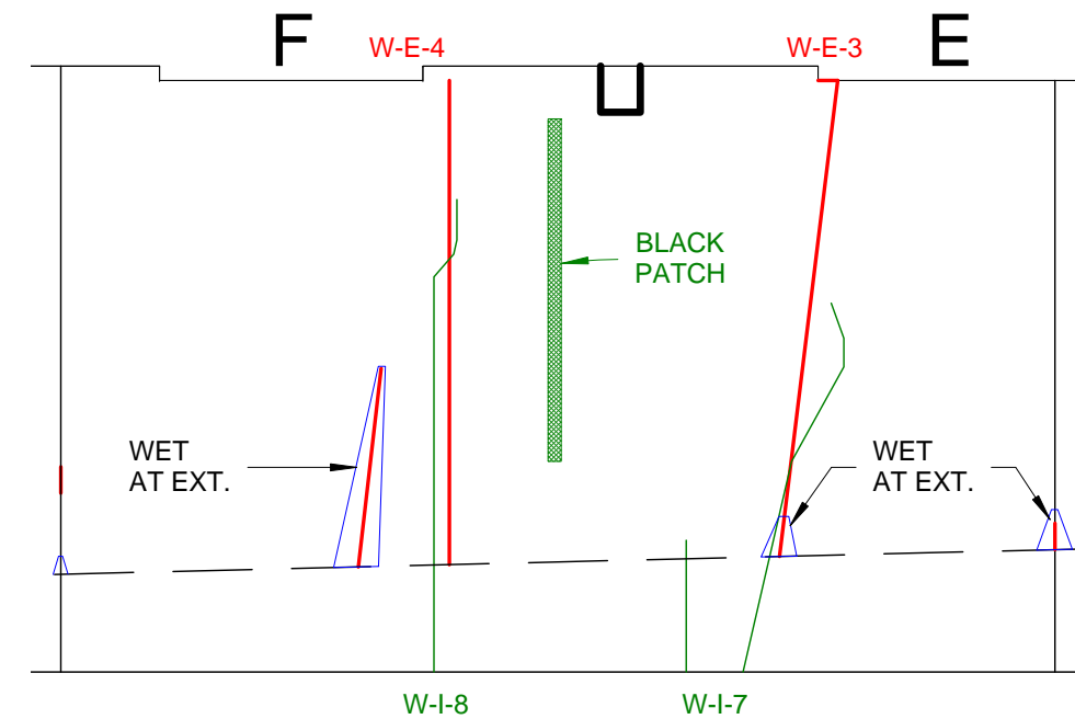
6 INT. PANEL 17 1/8" = 1'-0"
