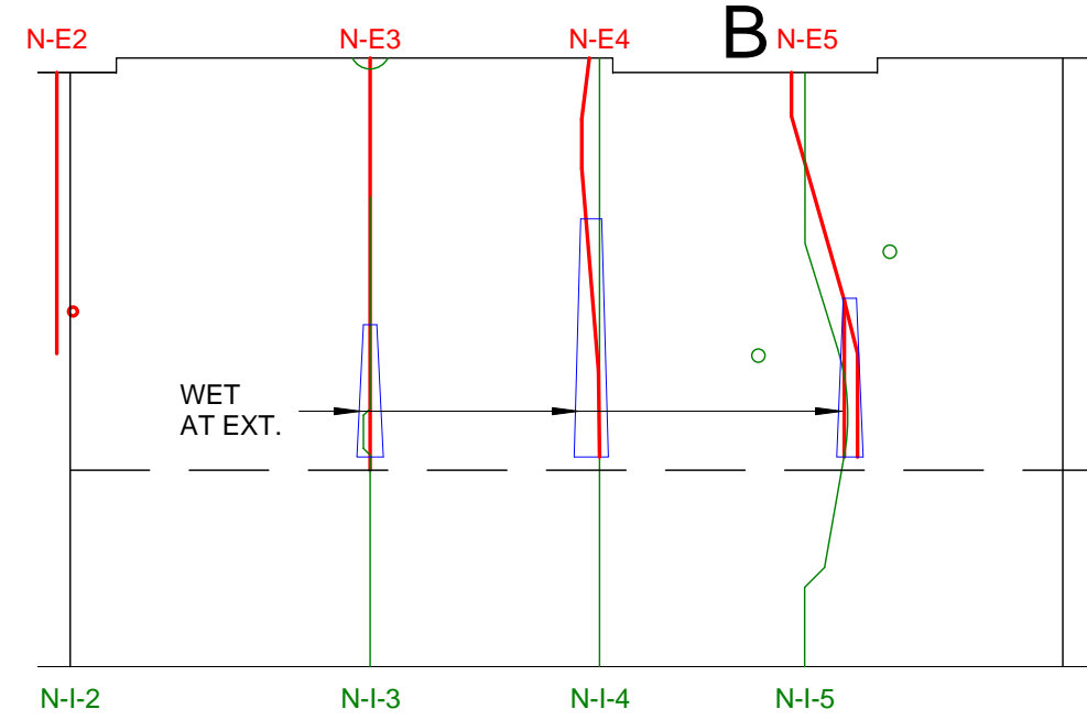
1 INT. PANEL 11 1/8" = 1'-0"
