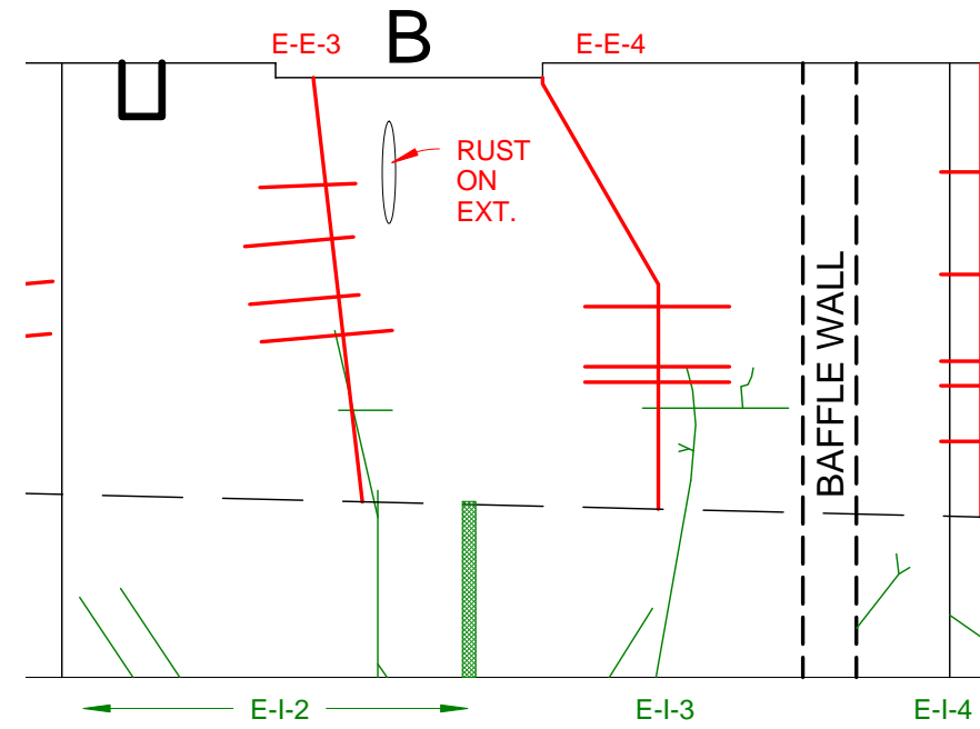
2 INT. PANEL 2 1/8" = 1'-0"
