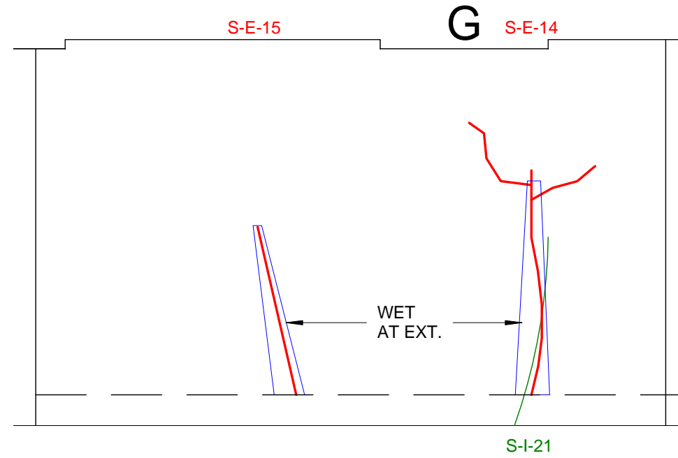
1 INT. PANEL 27 1/8" = 1'-0"
