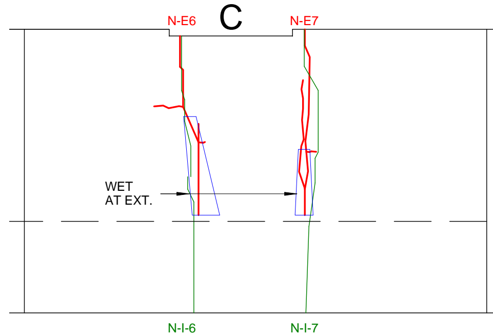
5 INT. PANEL 10 1/8" = 1'-0"
